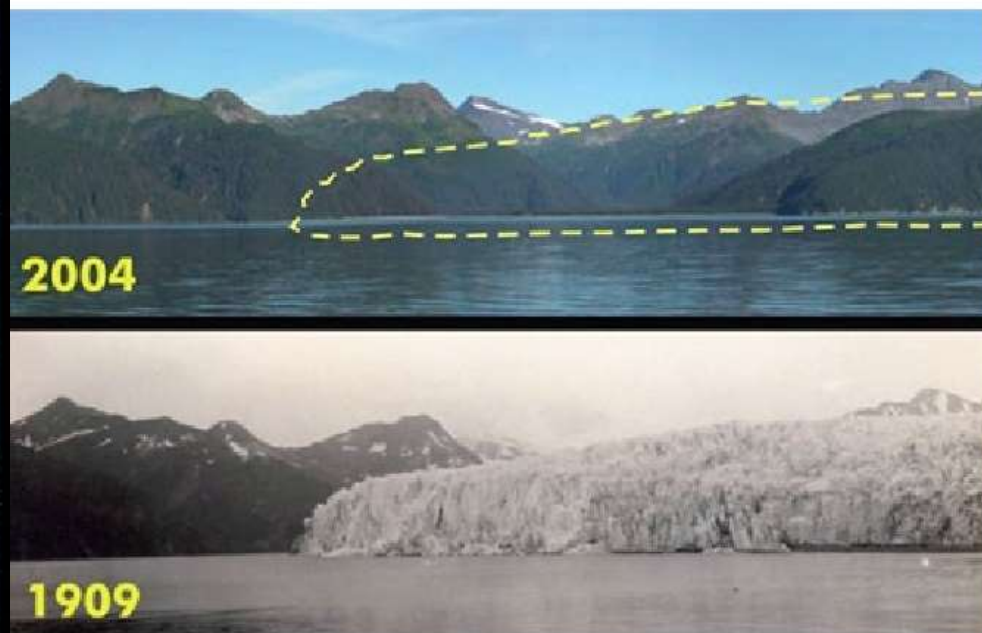
McCarty Glacier in Alaska
